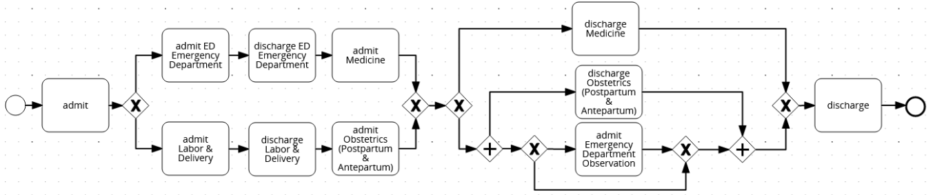
Fig. 8: The discovered process model illustrated as BPMN after applying the Inductive Visual Miner algorithm. For simplicity reason several activities are excluded from the process model
